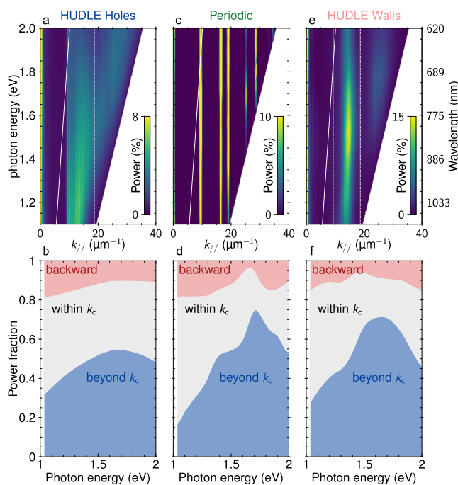
Figure 5. Momentum-resolved light trapping analysis of complete patterns. (a,c,e) Simulated power distribution of light transmitted through a semi-infinite air–Si interface as a function of in-plane momentum and photon energy for the HUDLE holes pattern (a, left), periodic (c, middle), and HUDLE walls (e, right). The white solid line represents the light line (critical angle) and vertical dashed lines denote in-plane momentum limits of the HUD design. (b,d,f) Integrated power fractions of light scattered by the nanostructures. Reflected power fraction (backward) shown in red at the top, power scattered into the escape cone (within k_c ) gray in the middle, and power scattered beyond the critical angle k_{\parallel} > k_c in blue at the bottom for HUDLE holes (b), periodic (d), and HUDLE walls (f) as a function of photon energy.
