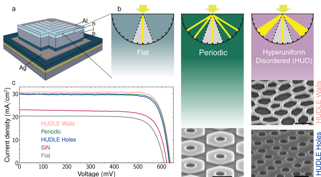
Figure 1. Schematic, operation principle, and performance metrics of 4.8 \mu\text{m} thick c-Si solar cell devices (a) Sketch of the 4.8 \mu\text{m} ultrathin solar cell device grown on a silicon-on-insulator (SOI) wafer with an initial seed layer thickness of 2 \mu\text{m} , on top of a 500 nm buried silicon dioxide layer separating the device from the 500 \mu\text{m} thick Si handle wafer. (b) Illustrative representation of light scattering and diffraction through different surface morphologies: flat (left), periodic nanopattern (middle), and hyperuniform disordered nanopattern (HUDLE, right). The corresponding scattering patterns into the substrate are highlighted as yellow lobes in the polar plots where the gray shaded area indicates the escape cone of light. Scanning electron micrographs of periodic and two HUDLE designs are also shown (scale bars: 500 nm). (c) Current–voltage characteristics obtained at 1-sun illumination for the best performing solar cell of each type.
