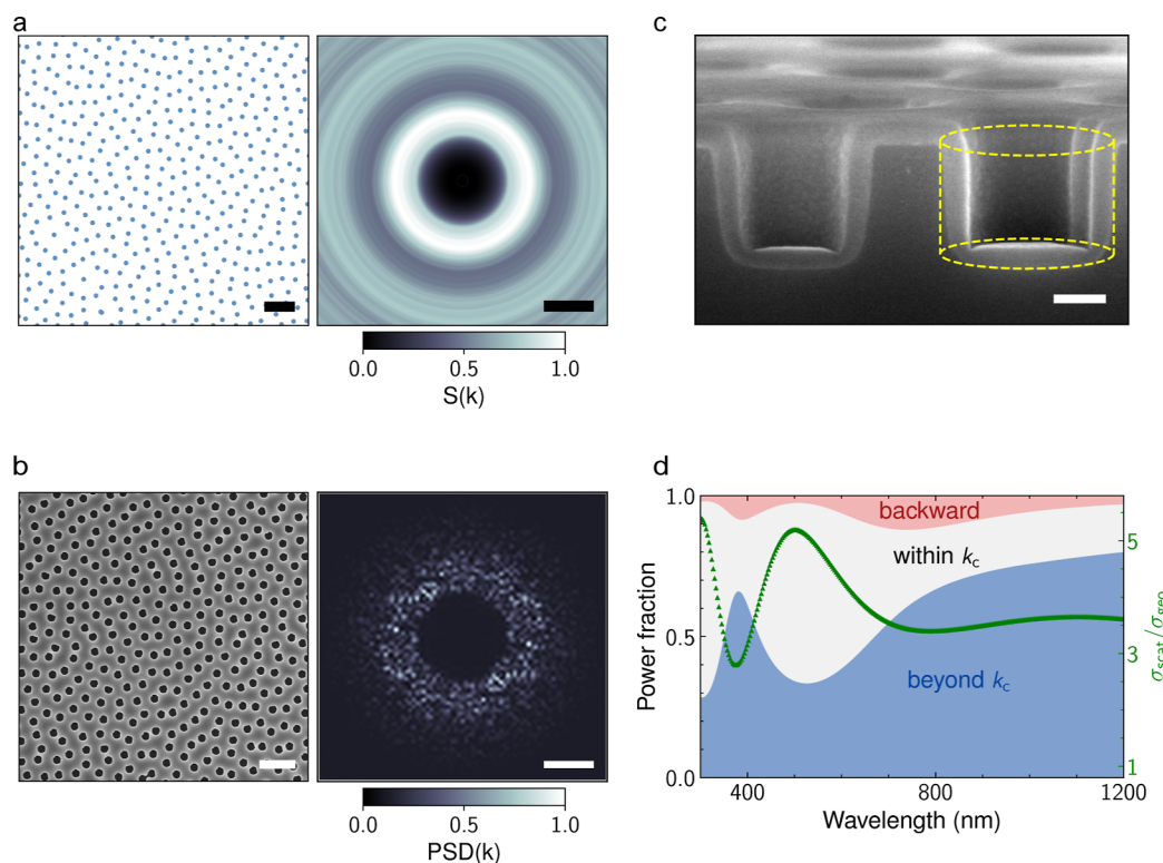
Figure 4. Light trapping mechanism of HUDLE layers. (a) HUDLE holes real space locations (left) and their corresponding structure factor S(k) (right). (b) SEM image of an as-fabricated HUDLE Holes pattern (left) and 2D fast-Fourier transform (FFT, right), obtained from it after Otsu thresholding and subtracting its mean intensity. Scale bars in (a, b) are 1\ \mu\text{m} and 10\ \mu\text{m}^{-1} for real- and Fourier space images, respectively. (c) Cross-sectional SEM image of the as-fabricated sample with the HUDLE hole pattern, where the scattering object is highlighted by a dashed frame and the scale bar is 100\ \text{nm} . (d) Scattering cross-section (green triangles) and direction-resolved scattered power fractions of a typical scattering object of the HUDLE holes pattern; a hole ( n = 1 ) coated with 55\ \text{nm} \text{SiO}_2 located at a silicon–air interface ( n_{\text{Si}} = 3.5 , k_{\text{Si}} = 0 ) of 180\ \text{nm} radius and 245\ \text{nm} height. Power fractions are displayed as shaded areas with reflection at the top (red), forward scattering into the escape cone ( k_{\parallel} < k_c ) in the middle (gray), and forward scattering beyond the critical angle ( k_{\parallel} > k_c ) at the bottom (blue).
