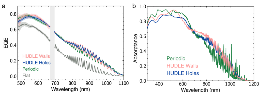
Figure 3. Spectral optoelectronic analysis. (a) Measured external quantum efficiency spectra of flat and patterned cells. The shaded regions around the curves indicate measurement uncertainty due to laser fluctuations, while the gray spectral region highlights the wavelength range that is inaccessible to our experimental setup. (b) Simulated absorbance of the corresponding device stacks.
