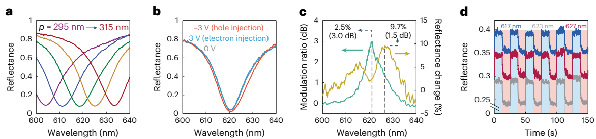
Fig. 3 | Intensity modulation of the reflected beam via electrical gating.
