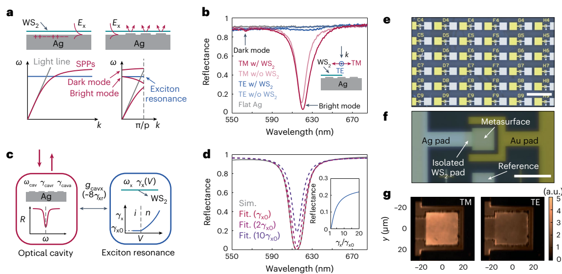
Fig. 2 | Enhanced modulation with a silver metasurface gate pad. a, Realization of a quasi-guided SPP mode supported by the metasurface gate pad following the introduction of a periodic perturbation to the top surface of the silver gate pad. Red curves represent the modal dispersion of the (perturbed) SPPs at the silver/dielectric interface, and grey lines refer to the light lines in the dielectric. Two optical modes are found at the \Gamma -point near the exciton resonant frequency supported by the silver metasurface gate pad. b, Measured reflection spectra of fabricated optical modulators under transverse-magnetic (TM) polarized (red) and transverse-electric (TE) polarized (blue) normal illumination. Solid and semi-transparent curves represent the reflection spectra for the devices with and without WS 2 monolayers, respectively. The grey curve indicates the reflection spectrum of the flat silver gate pad. c, Mechanism of the
