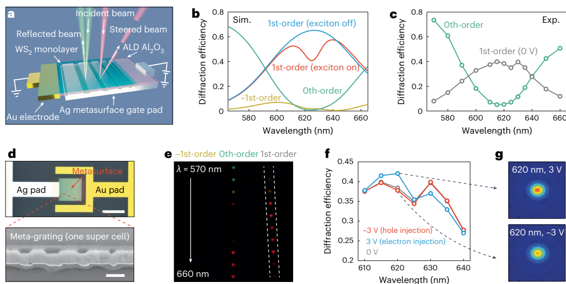
Fig. 4 | Monolayer WS 2 light-field modulators with a beam-steering function.
