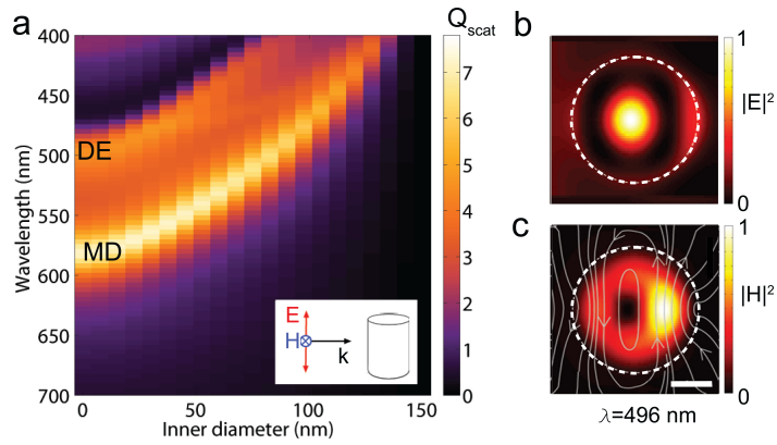
Fig. 12. Simulated normalized scattering cross section ( Q_{sc} ) of a 150 nm diameter and 100 nm tall Si cylinder in air, as function of wavelength and gap width in the visible wavelength range. The modes were excited with a vertically polarized plane wave (with the E -field along the long axis of the particle), as seen in the inset of (a). The normalized electric (b) and magnetic (c) field intensity profiles for a solid particle with no gap with the corresponding electric field lines are shown for the xy -plane in the center of the particle on resonance, where the particle contour is plotted as white dashed lines. The field intensities are normalized to its maximum values. The scale bar in (c) represents 50 nm.
